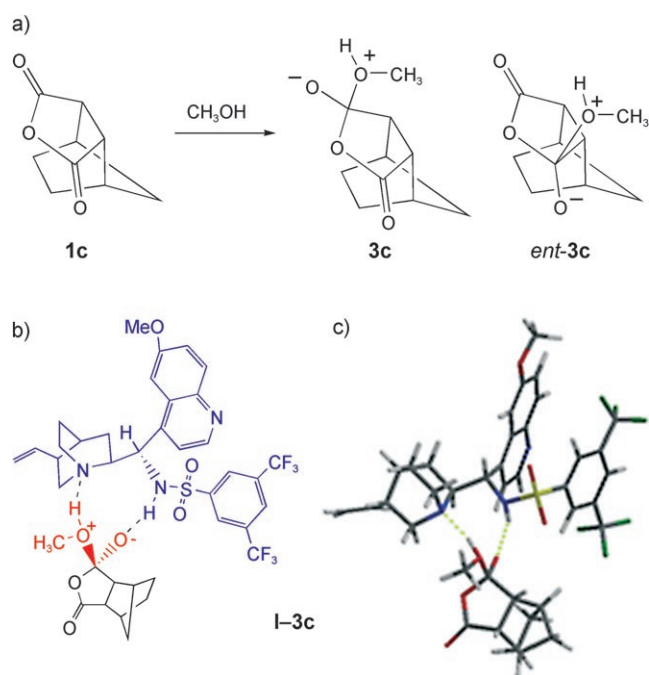
Scheme 3. a) Transition-state analogues 3c and ent-3c for the non-catalyzed methanolysis reaction. b) Schematic representation of the catalyst-transition-state-analogue complex I–3c , which gives the major product. c) Computed structure of I–3c . [15]
